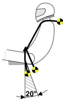
SHOULDER BELT ANGLE
